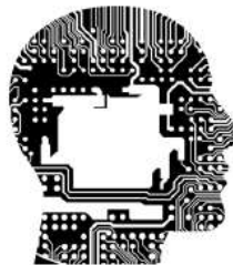
AI development
