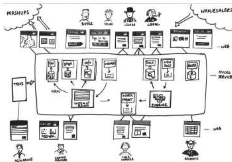
Microservice architecture
